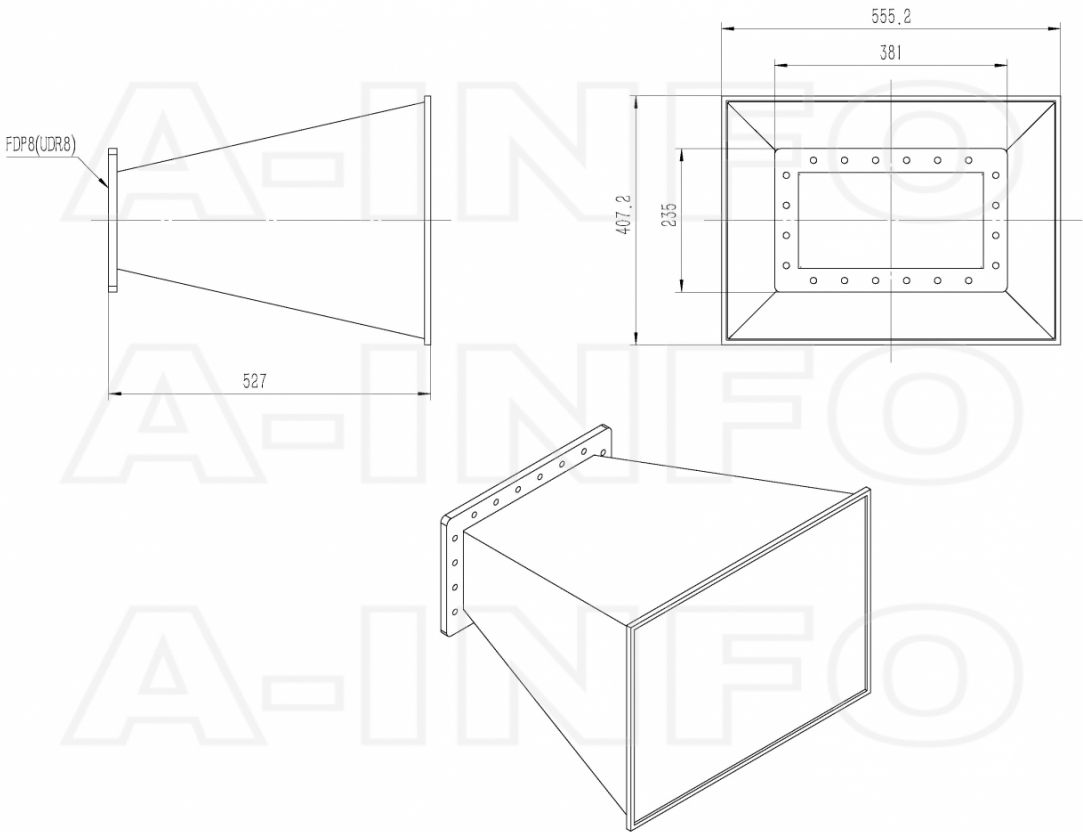
FDP8 Output with Radome (Option, P/N: LB-1150-10-ASPO, Outdoor Application)
