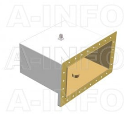
1150WCANM Right Angle Rectangular Waveguide to Coaxial Adapter 0.64-0.96GHz WR1150 to N Type Male
